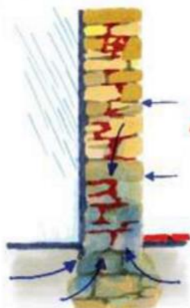
CAPILLARITE
